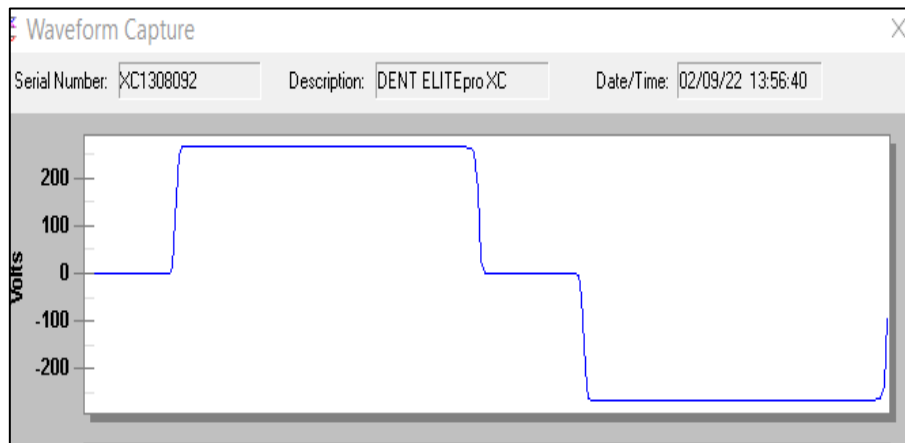
Figure 5: Voltage Waveform of the Inverter Output
