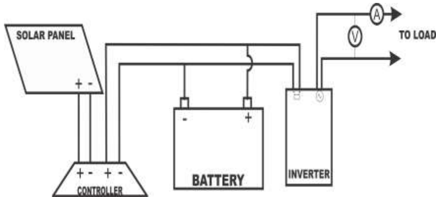
Figure 3: Experimental Set-up for the Research
