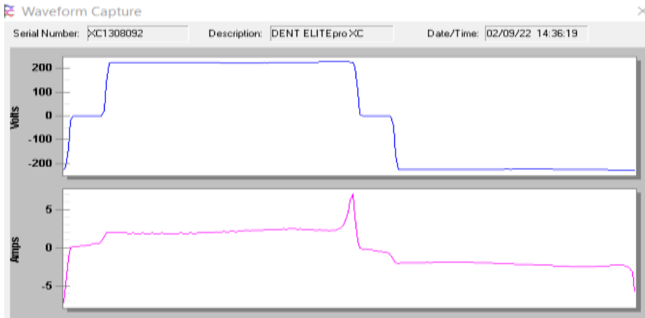
Figure 9: Voltage and Current Waveforms of the Inverter Under Load Case 2
