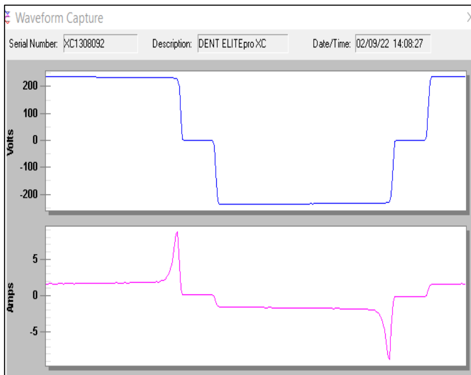
Figure 7: Voltage and Current Waveforms of the Inverter Output
