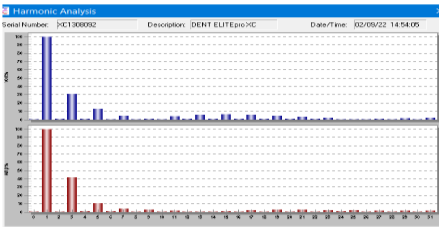
Figure 12: Voltage and Current Harmonics Spectrum of Inverter Under Load Case 3
