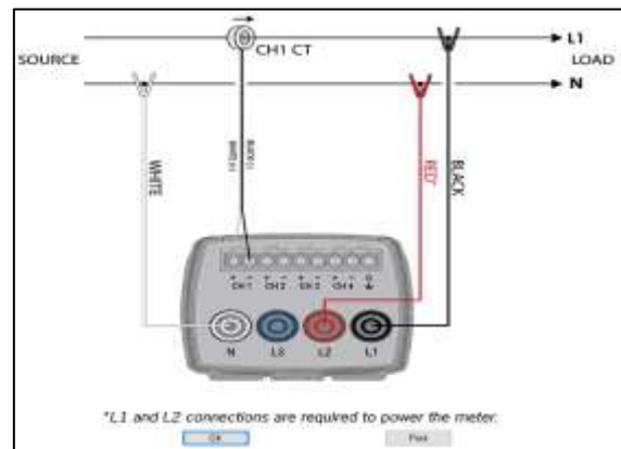
Figure 4: Typical Connection for the DENT Power Meter Used for the Harmonic Evaluation
