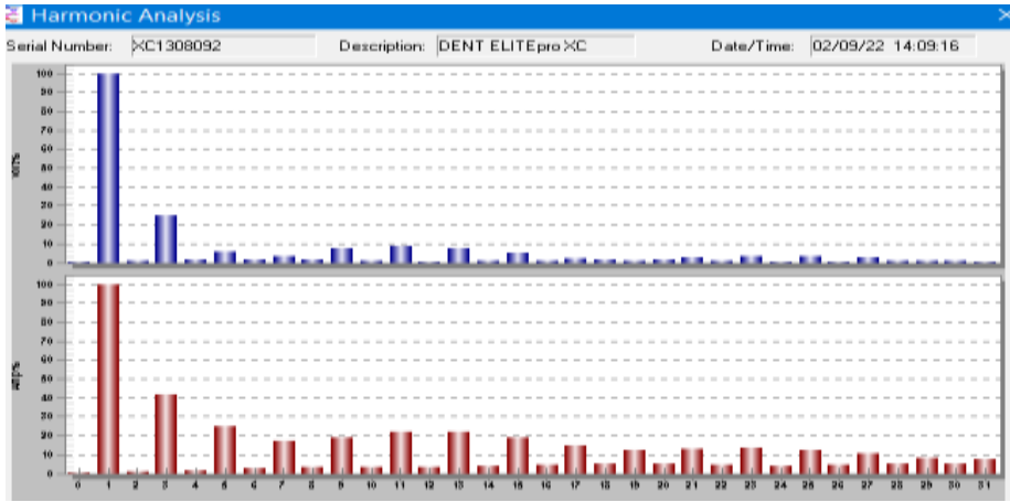
Figure 8: Harmonics Spectrum of Voltage and Current Output of the Inverter
