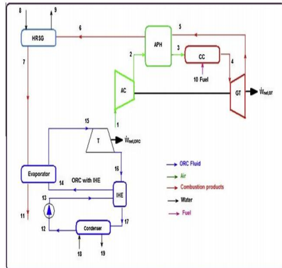
Fig 1: Schematic Diagram of GT-HRSG/ORC System [4]
