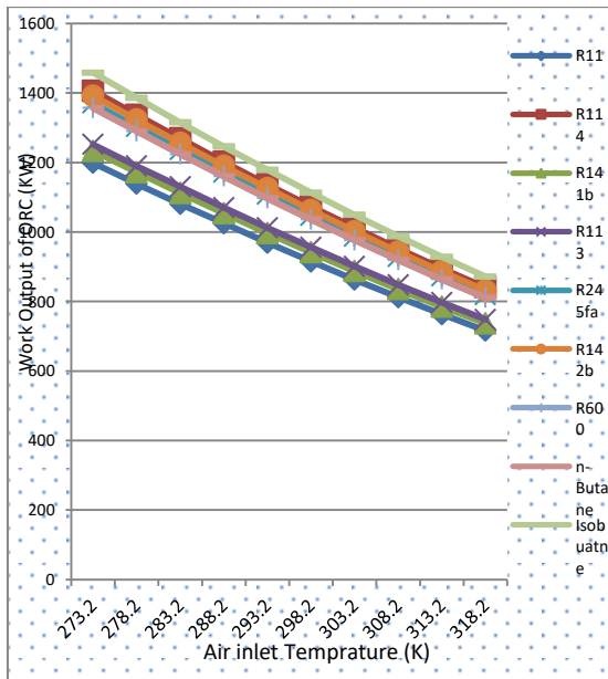
Fig 3: Comparison of Performance of Various Organic Fluid Operating in Bottoming Cycle of Cogeneration System
