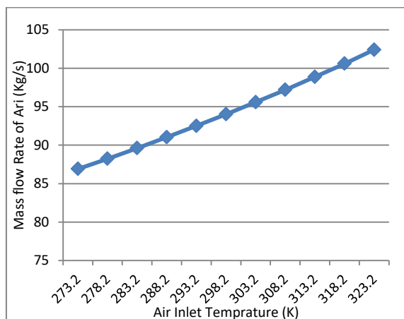
Fig 2 (c): Variation of Mass Flow Rate of Air with Surrounding Temperature
