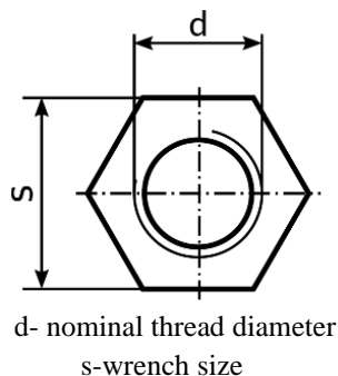
Figure 1: Hexagon of a Screw with Wrench Size “s” and Nominal Thread Diameter “d” [12].
