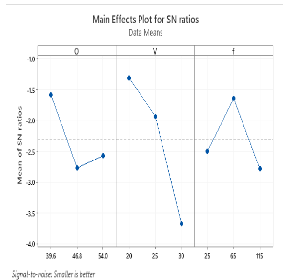
Figure 7: Effects of Overhanging of Tool, Cutting Speed and Feed Rate on S/N Ratio
