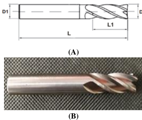
Figure 4: (A) Parallel Shank 4F Endmill with Designated Dimensions [15], (B) Cutting Tool Used for Experimental Runs
