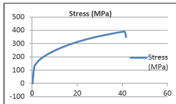
Fig 3: Stress Vs Strain Curve of 304-304 Combination
