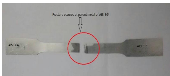
Fig 11: AISI 304-316 Specimen After Tensile Test
