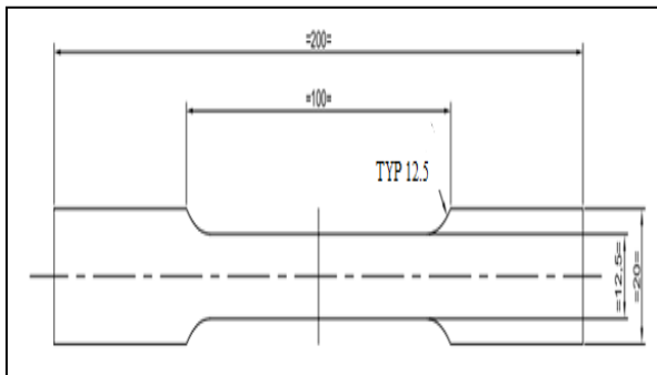
Fig 1: Dimension of Specimen
