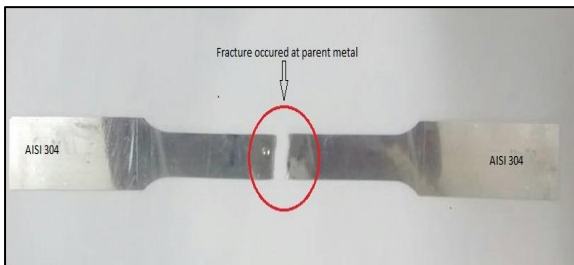
Fig 5: AISI 304-304 Specimen After Tensile Test
