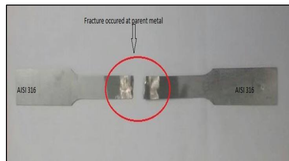
Fig 8: AISI 316-316 Specimen After Tensile Test
