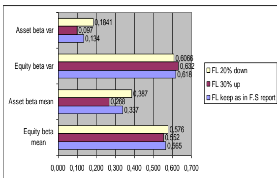
Fig.2. Comparing Statistical Results of Three (3) Scenarios of Changing FL (Period 2007-2011)
