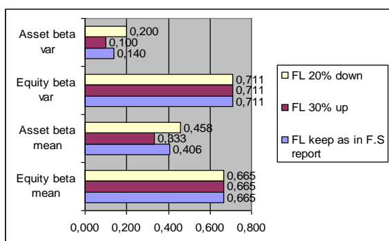
Fig.2. Comparing Statistical Results of Three (3) Scenarios of Changing FL (Period 2007-2011)
