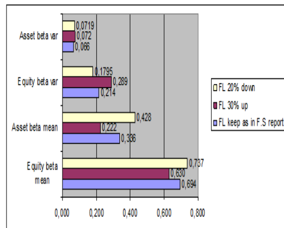
Fig4: Comparing Statistical Results of Three (3) Scenarios of Changing FL of 121 Listed Firms in the Consumer Good Industry
