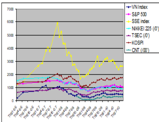
Fig.3.VNI Index and Other Stock Market Index During Crisis 2006-10
