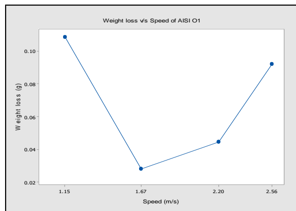
Fig 1(b): Friction Behaviour of AISI O1
