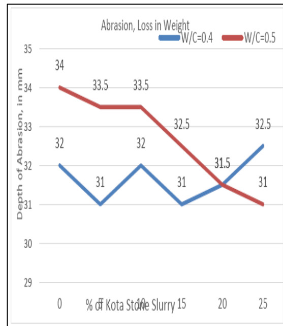
Fig 10: Depth of Abrasion, Abrasion Test
