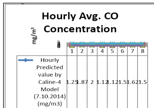
Fig 10: 8 hrs. Avg. Co Concentration
