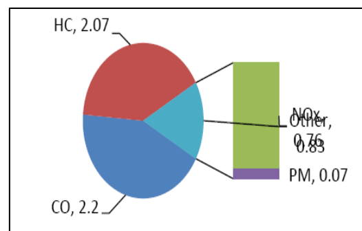
Fig 5: Average Weighted Emission Factor (g/km/Vehicle)
