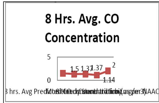
Fig.9: 8 hrs. Avg. Co Concentration
