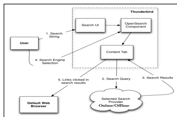
Fig 1: Process of Search Engine
