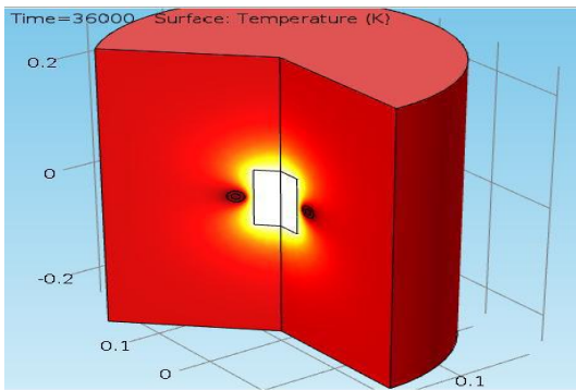
Fig 6: Surface Temperature of Cylinder after 10 hrs.
