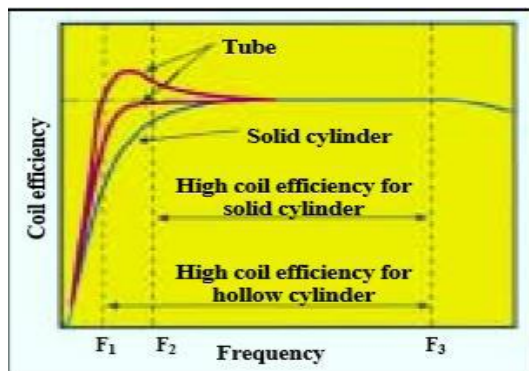
Fig 5: Graph Coil Efficiency vs. Frequency Conditions for Maximizing the Electrical Efficiency of the Induction Coil are Different for Tubes and Solid Cylinders. [9]
