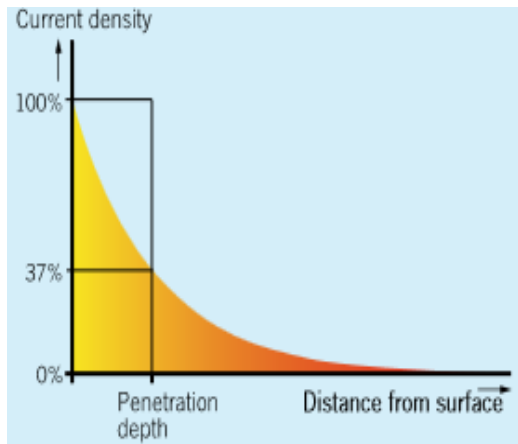
Fig 3: Graph Current Density Vs Distance from Surface [9]
