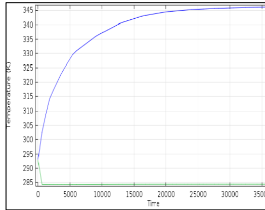
Fig 8: Point Graph Temperature (K)
