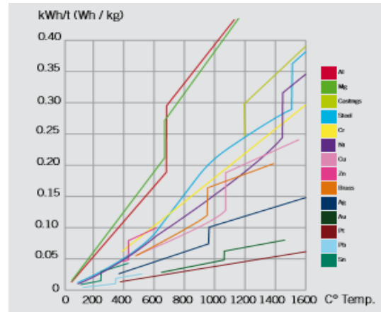
Fig 4: Energy Requirement Rate for Different Materials [9]
