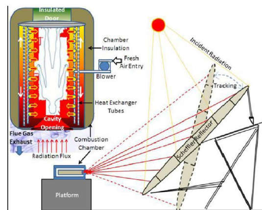
Fig 1: Block Diagram of Solar Crematorium
