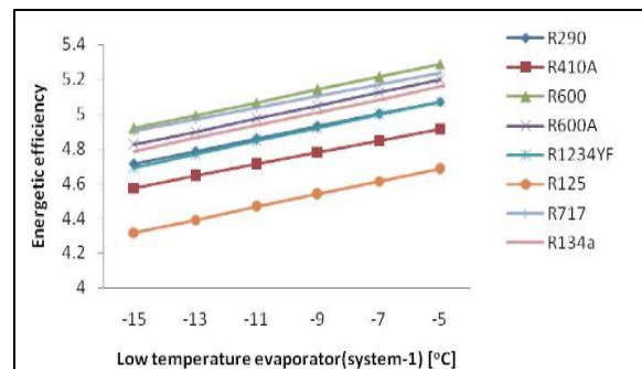
Fig 3: Variation of Low Temperature Evaporator of System-1 with Energetic Efficiency
