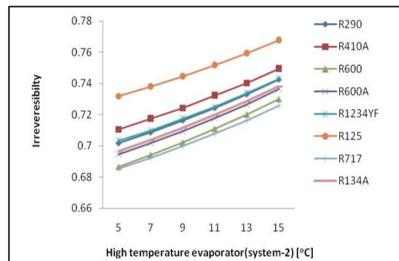
Fig 20: Variation of High Temperature Evaporator with Irreversibility of Sytem-2
