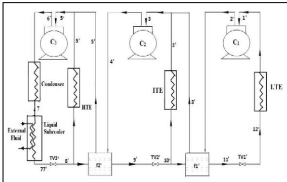
Fig 2: Schematic Diagram of Multiple Evaporators with Compound Compression, Flash Intercooler and Multiple Throttle Valves
