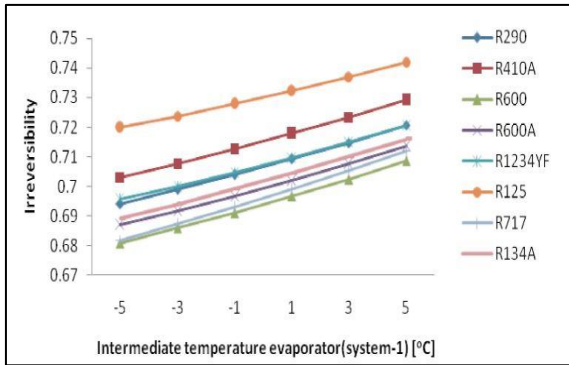
Fig 17: Variation of High Temperature Evaporator with Irreversibility of Sytem-1
