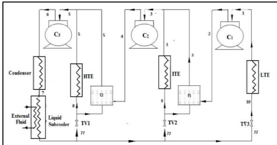
Fig 2: Schematic Diagram of Multiple Evaporators with Compound Compression, Flash Intercooler and Multiple Throttle Valves
