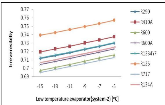
Fig 18: Variation of Low Temperature Evaporator with Irreversibility of Sytem-2
