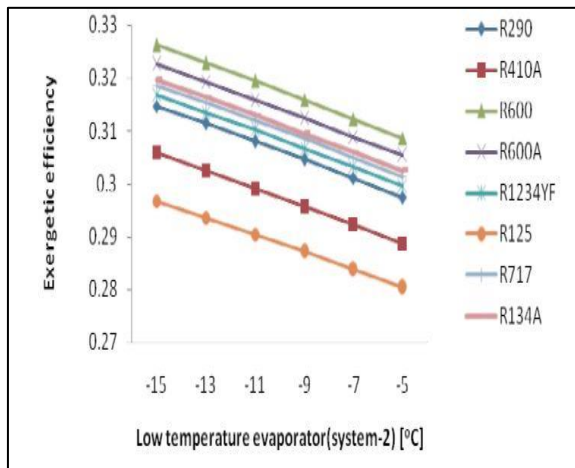
Fig 12: Variation of Low Temperature Evaporator of System-2 with Exergetic Efficiency
