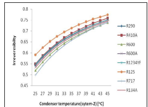
Fig 26: Variation of Condenser Temperature with Irreversibility of Sytem-2
