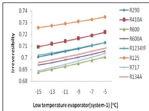
Fig 15: Variation of Low Temperature Evaporator with Irreversibility of Sytem-1
