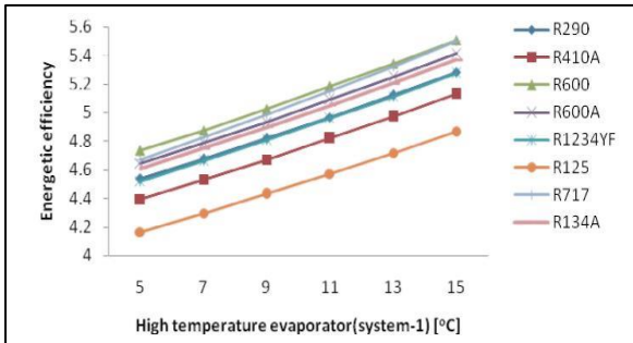
Fig 4: Variation of Intermediate Temperature Evaporator of System-1 with Energetic Efficiency
