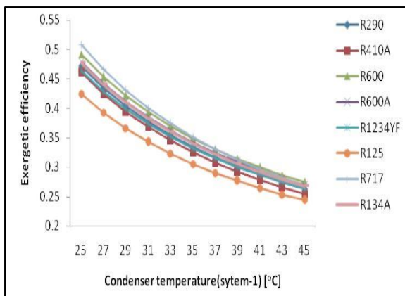
Fig 23: Variation of Condenser Temperature with Exergetic Efficiency of Sytem-1
