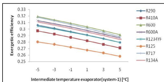
Fig 10: Variation of Intermediate Temperature Evaporator of System-1 with Exergetic Efficiency
