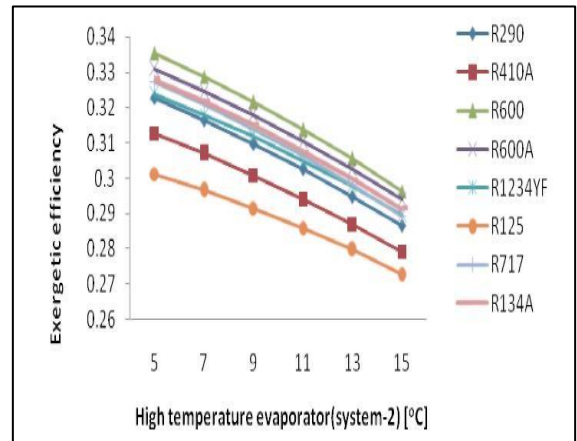
Fig 14: Variation of High Temperature Evaporator of System-2 with Exergetic Efficiency
